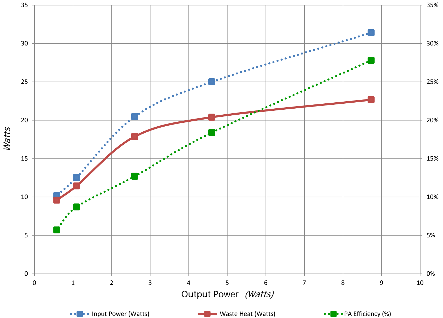
Elecraft® KX3 52 MHz PA Behavior – Measurements Courtesy of 5B4AIY
