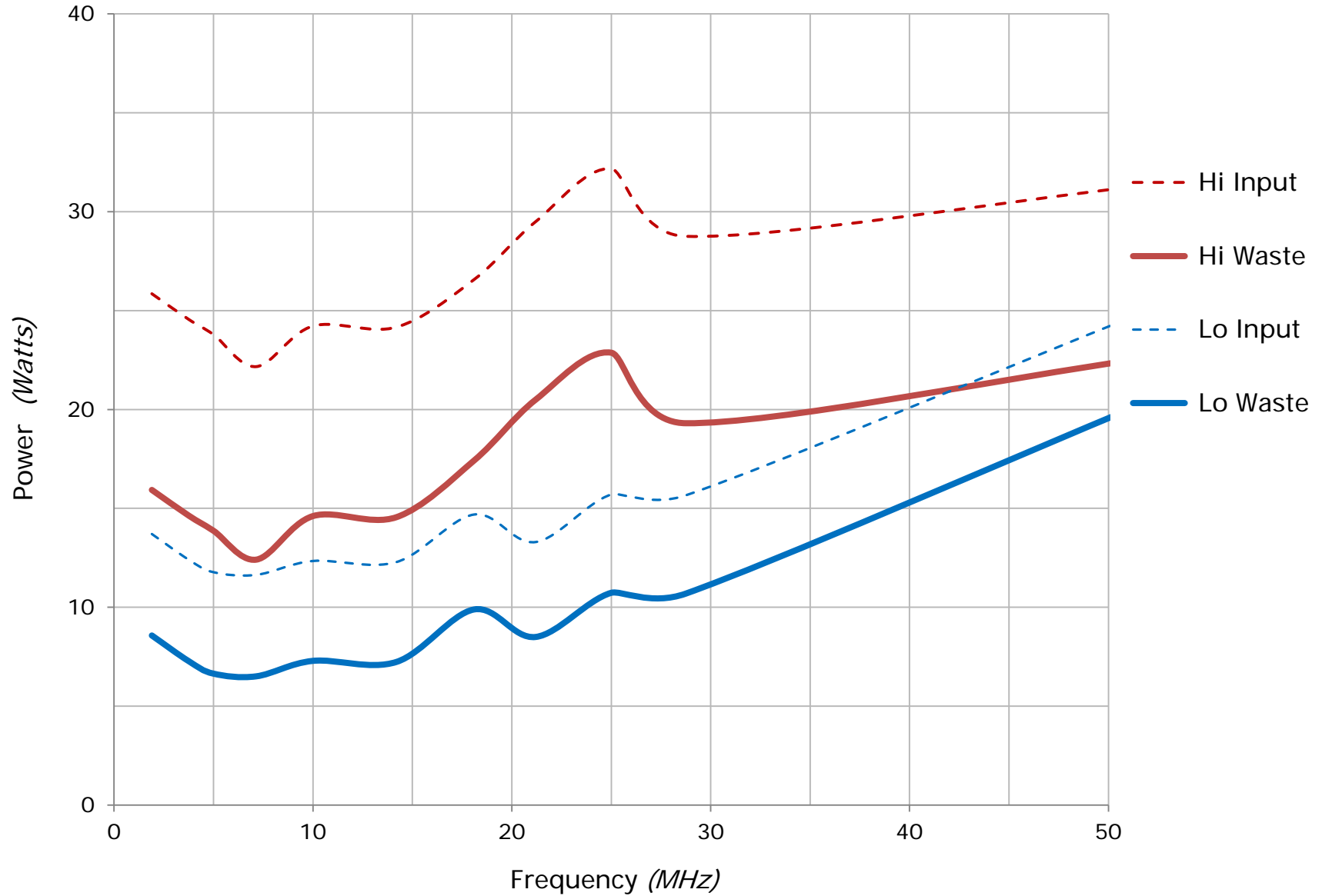
Input Power & Waste Heat as A Function of Frequency
